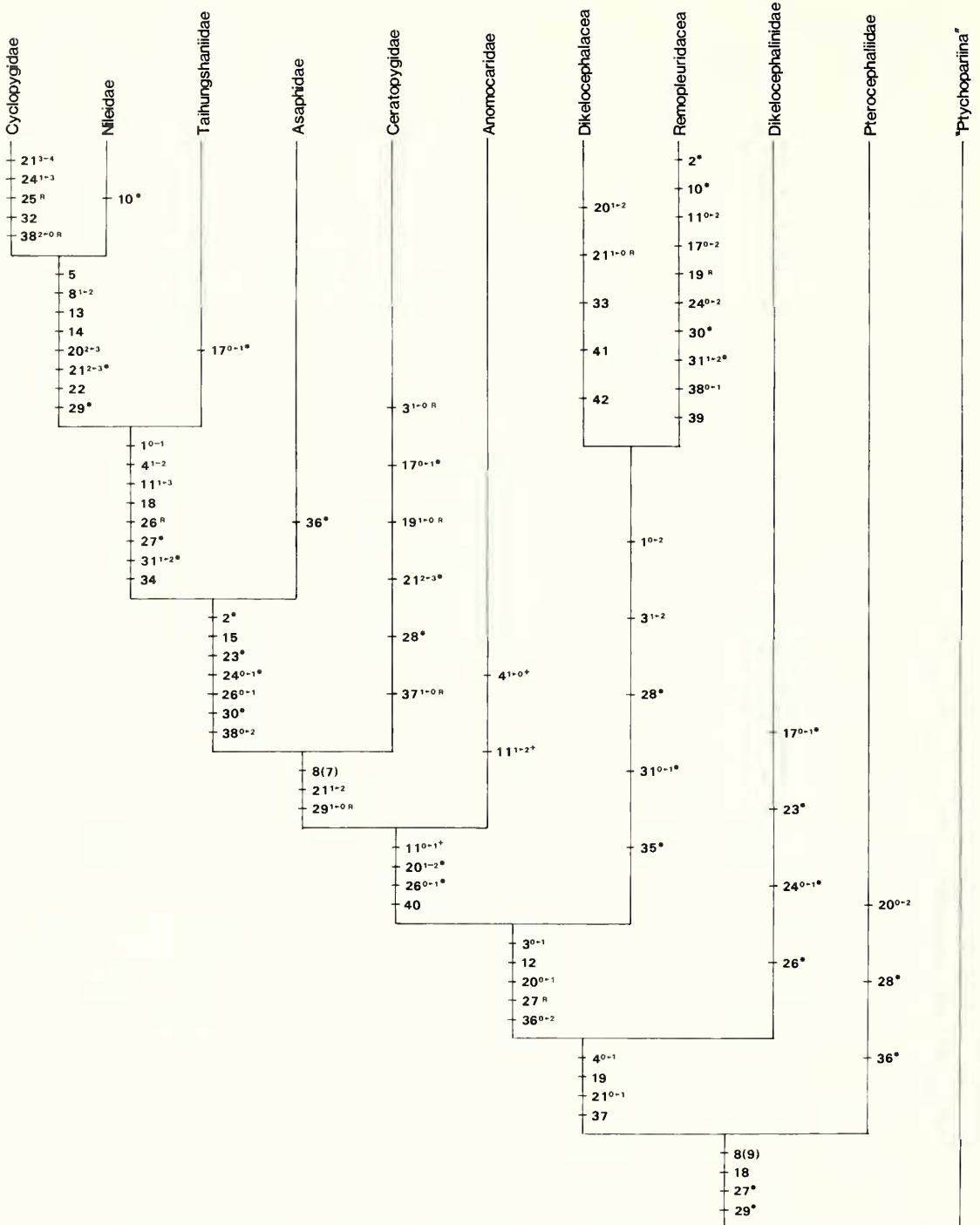
TEXT-FIG. 2. Cladogram produced from the PAUP computer analysis of the characters given in Table 2. Another equally parsimonious cladogram is shown in text-fig. 3. Note that text-figs. 2 and 3 resemble each other, apart from the position of Dikelocephalinidae and Pterocephaliidae. Pterocephaliidae and Anomocaridae are coded separately (cf. text-fig. 1) rather than included in 'Anomocaracea' sensu lato . Numbering of characters as in Table 2. Direction of character transformation for multistate characters is indicated. For symbols see text-fig. 3.
